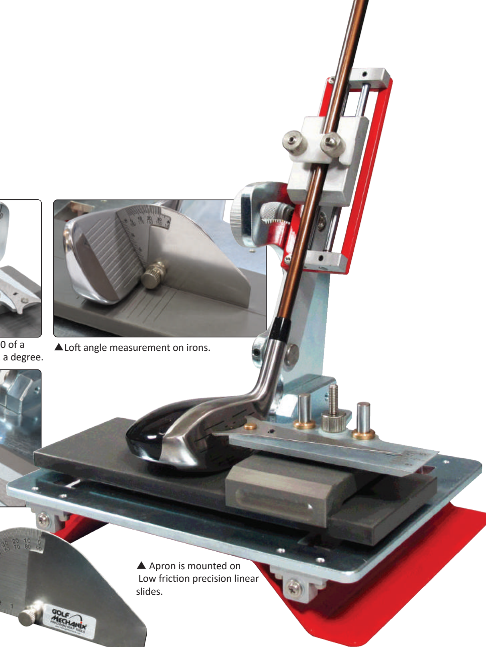
▲ The apron and base provide two reference planes from which an accurate setup can be achieved.
