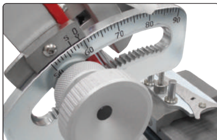
▲ Vernier style fractional scale with 1/10 of a degree accuracy and a resolution of 1/2 a degree.
